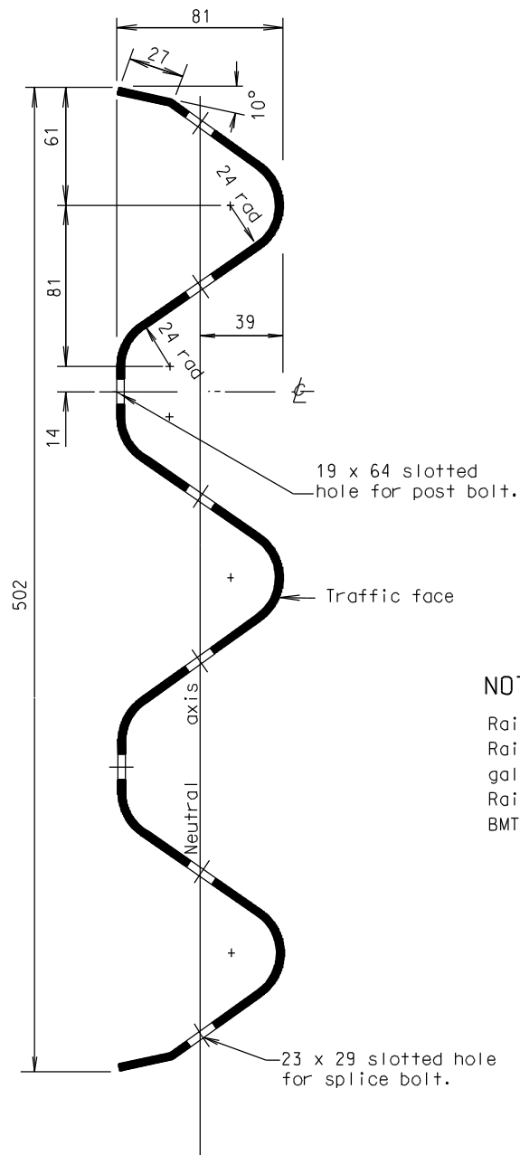
STIFFENER (B004)
